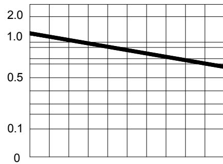
Fig.3 Relative Luminous Intensity vs Ambient Temperature
